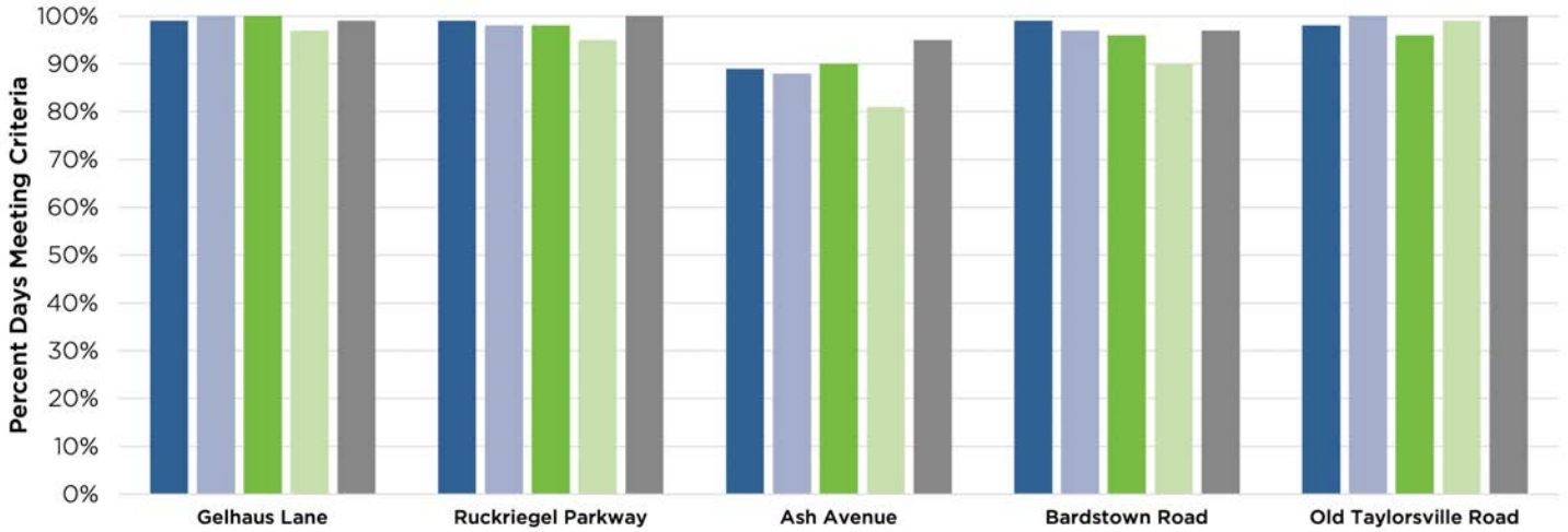
Dissolved Oxygen in Floyds Fork Watershed Water Years (October 1 to September 30)
